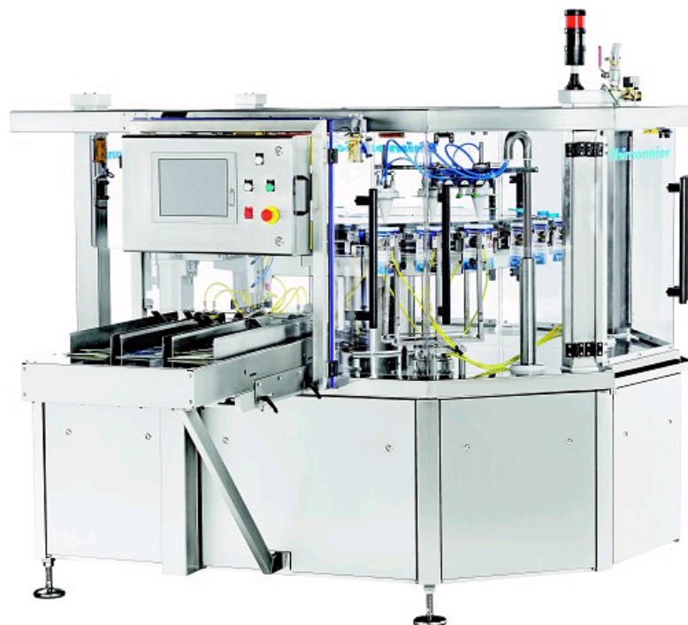
FULL MECATRONIC TECHNOLOGY DOYPACK® (STAND-UP POUCHES) MACHINE
