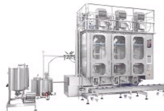
HIGH SPEED ASEPTIC VERTICAL FFS MACHINE
