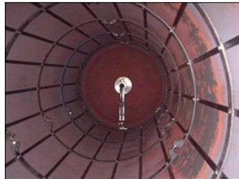
TURBULATOR BARS FOR PAPER MACHINE CYLINDER'S DRYERS
