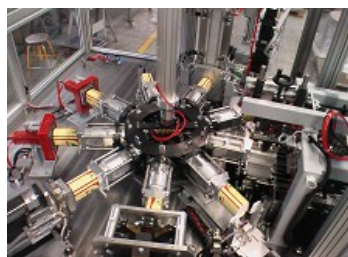
PRISMAPAK, MACHINE MANUFACTURING PACKAGING CARDBOARD SINGLE-WRAP
