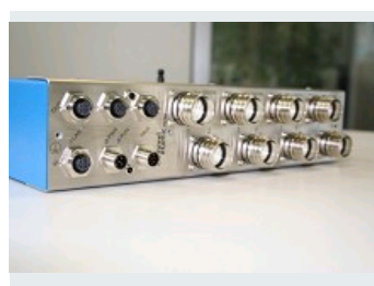
THE PS-100 ROBUST (IP54) PROBE SATELLITES (8 TO 16 PROBES).
