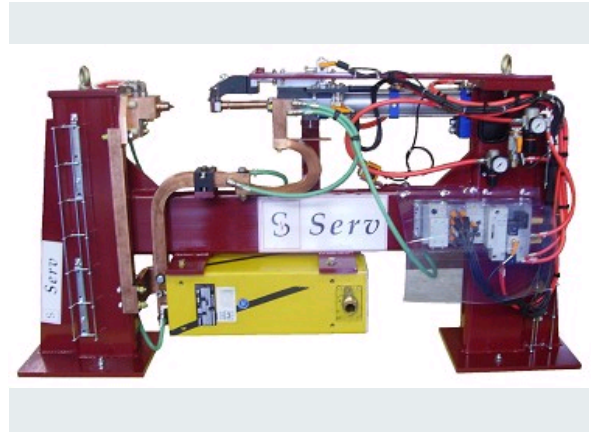
AUTOMATIC NUT WELDING
