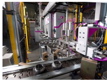
LASER WELDING LINE
