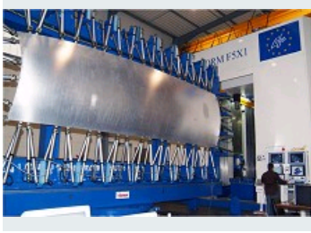
AERO: MILLING MIRROR SYSTEM TECHNOLOGY WORLD LEADER IN ALUMINIUM FUSELAGE SKIN MACHINING. PATENTED CONCEPT
