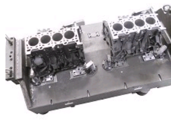
WORKPIECE CLAMPING FIXTURE
