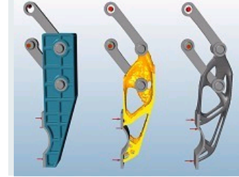
TOPOLOGICAL OPTIMIZATION OF PARTS PRODUCED IN ADDITIVE MANUFACTURING
