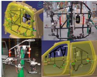
PNEUMATIC STANDALONE JIGS FOR METAL LINE
