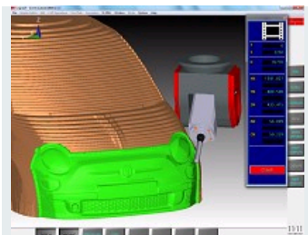
VIMILL LOOK AHEAD VIRTUAL MILLING IN 5 AXIS
