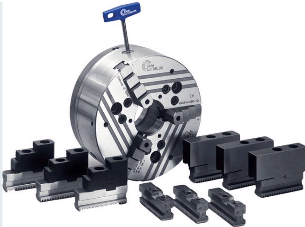
QUICK JAW CHANGE POWER CHUCKS
