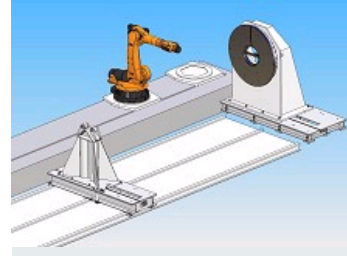
20 T PLATE, BED & FOLLOX REST DESIGN AND MANUFACTURE TOOLING FOR WORPIECE HOLDER
