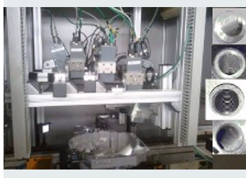
IDENTIFICATION - CONTROL DRILLING / TAPPING
