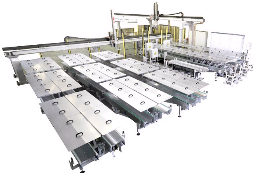
HANDLING AND STORAGE OF ENGINE HEADS BETWEEN MACHINING AND ASSEMBLY LINES
