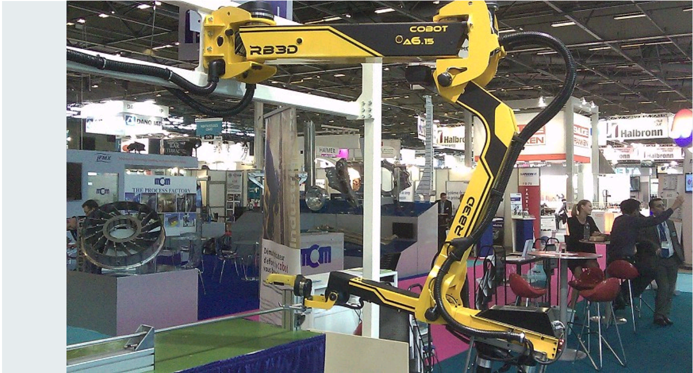
6 AXIS COLLABORATIVE ROBOT
